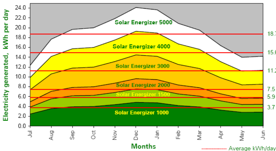
Estimated Daily Energy Production* (Sydney Australia)
